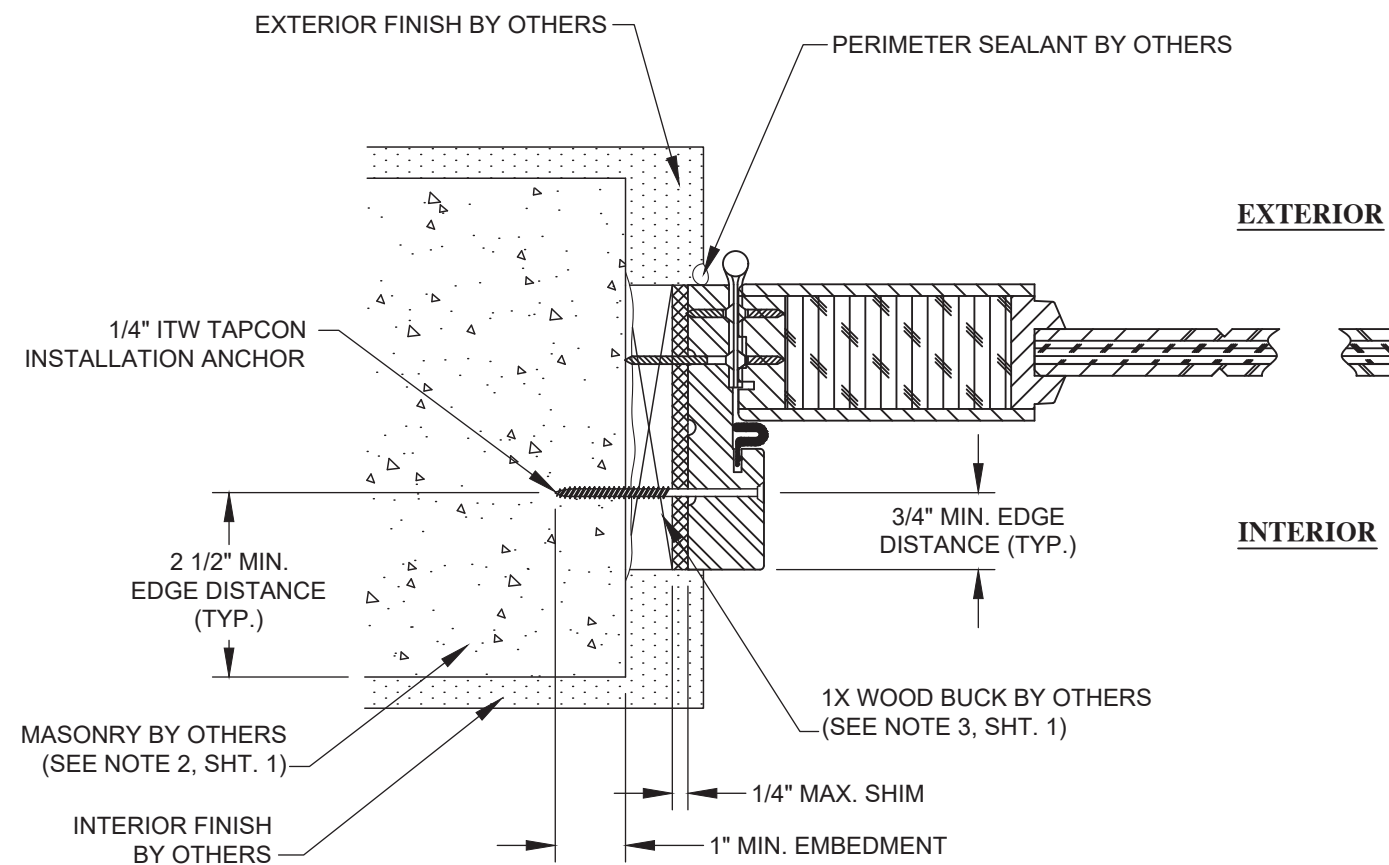
N 11 HORIZONTAL SECTION MASONRY SUBSTRATE STANDARD DESIGN JAMB FRAME
