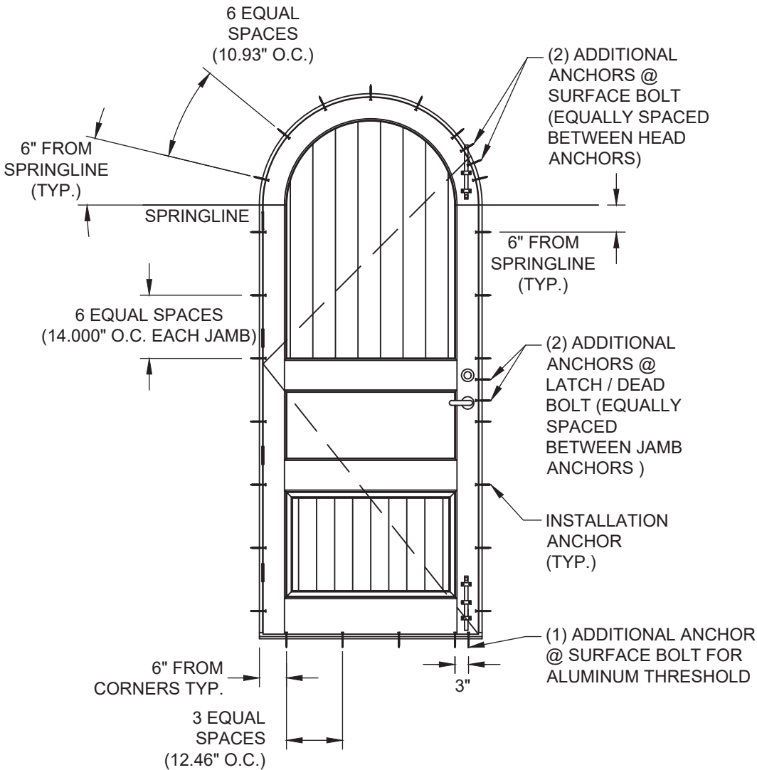
ANCHOR LAYOUT 1 INTERIOR VIEW
