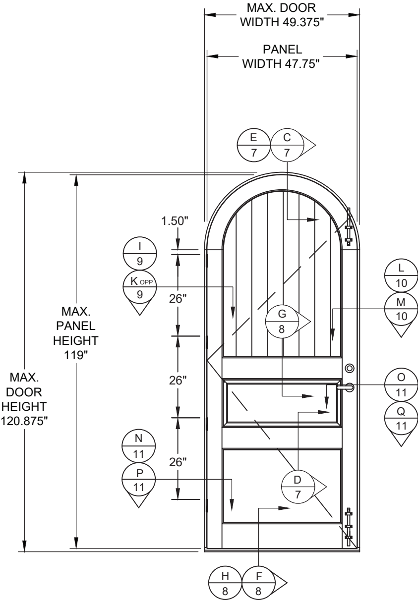
ELEVATION 1 INTERIOR VIEW
