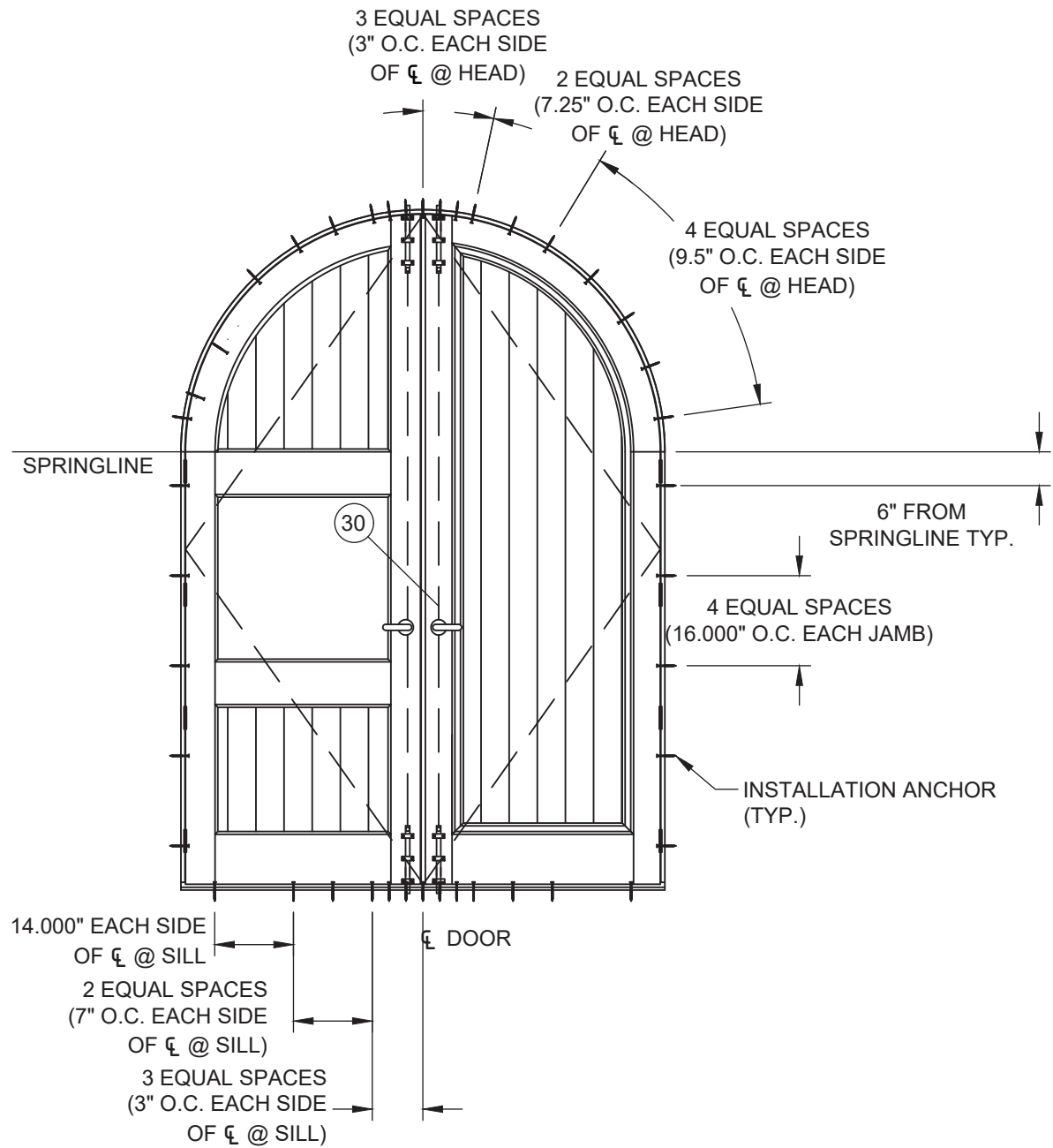
ANCHOR LAYOUT 2
