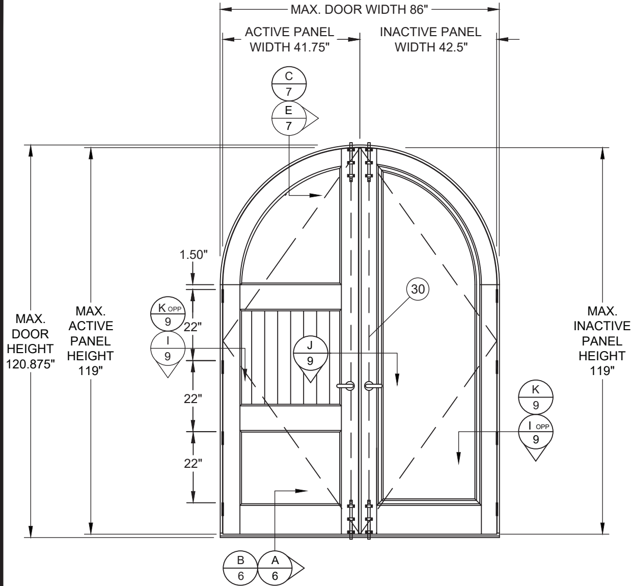
ELEVATION 2 INTERIOR VIEW
