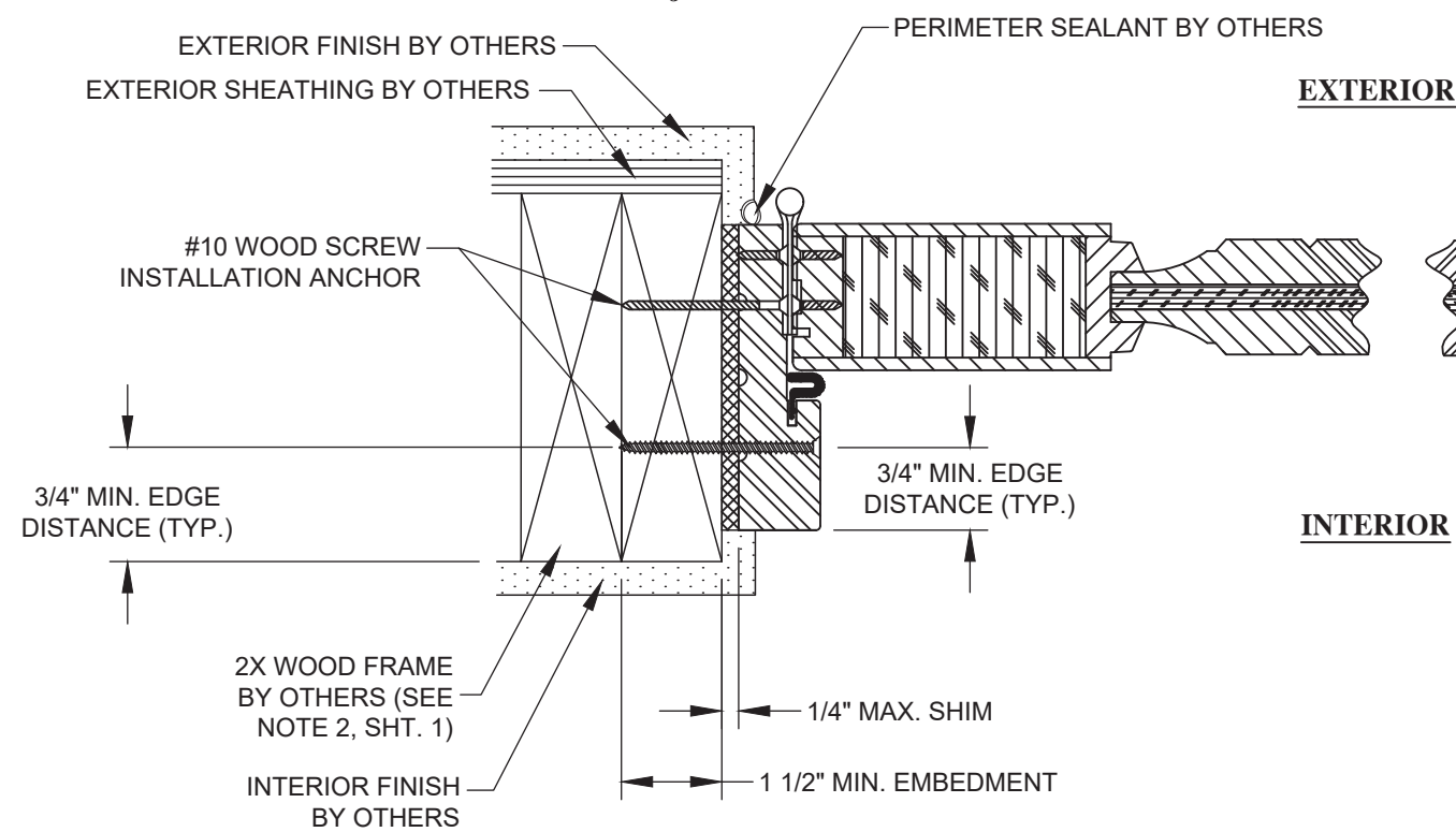
P HORIZONTAL SECTION 11 WOOD FRAME SUBSTRATE STANDARD DESIGN JAMB FRAME
