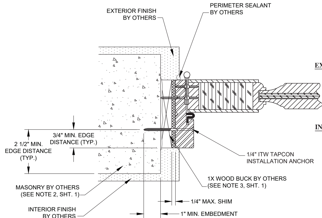
I 9 HORIZONTAL SECTION MASONRY SUBSTRATE EURO DESIGN JAMB FRAME
