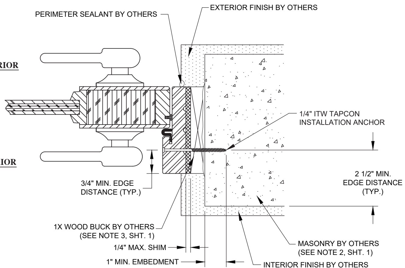
011 HORIZONTAL SECTION MASONRY SUBSTRATE STANDARD DESIGN JAMB FRAME
