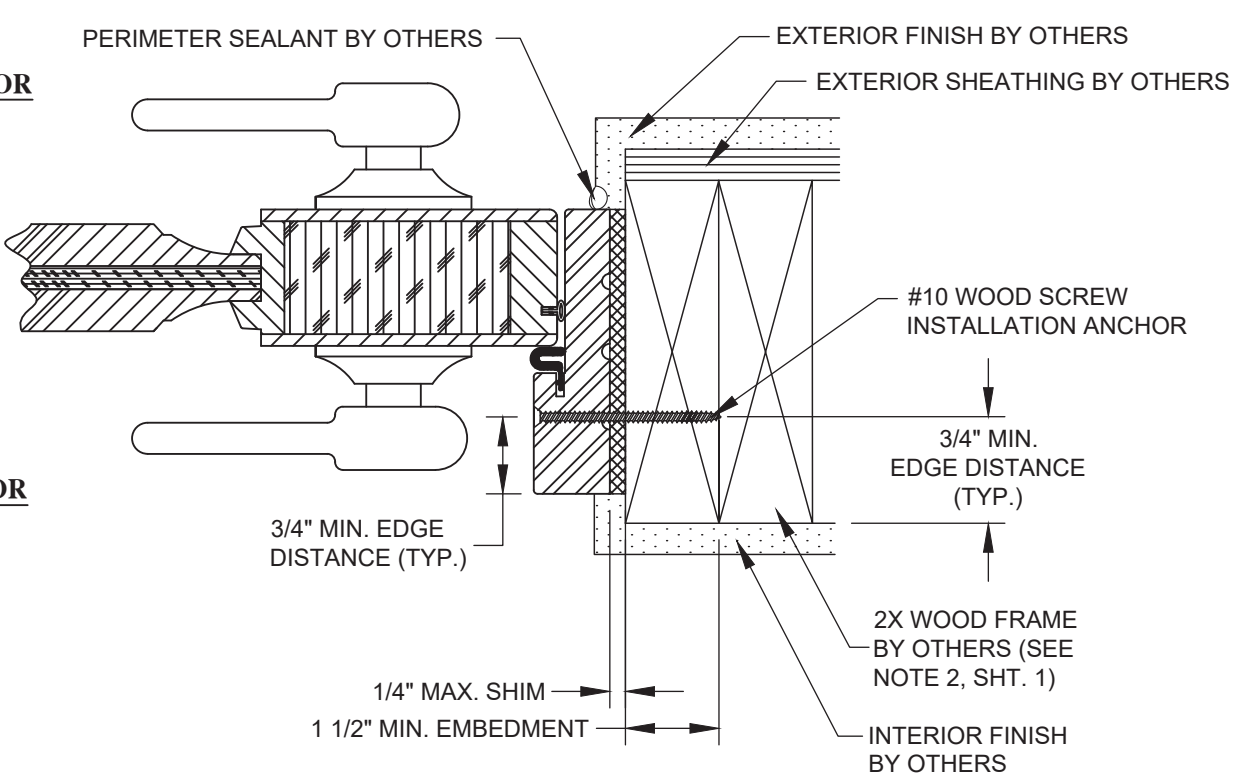
Q11 HORIZONTAL SECTION WOOD FRAME SUBSTRATE STANDARD DESIGN JAMB FRAME
