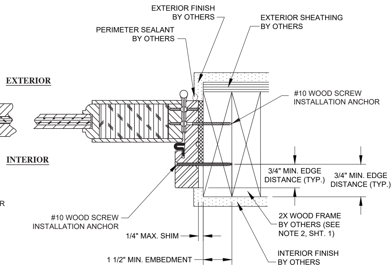
K 9 HORIZONTAL SECTION WOOD FRAME SUBSTRATE STANDARD DESIGN JAMB FRAME
